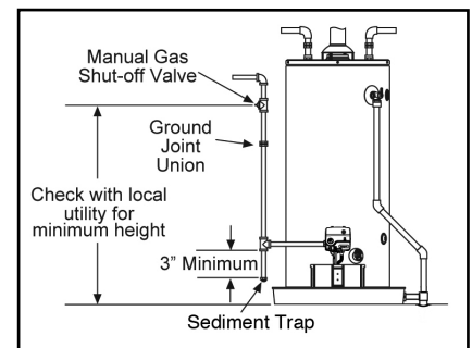
Figure 4: Gas Piping
